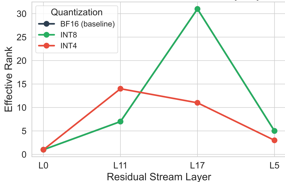
Arithmetic Manifold: Effective Rank by Layer
