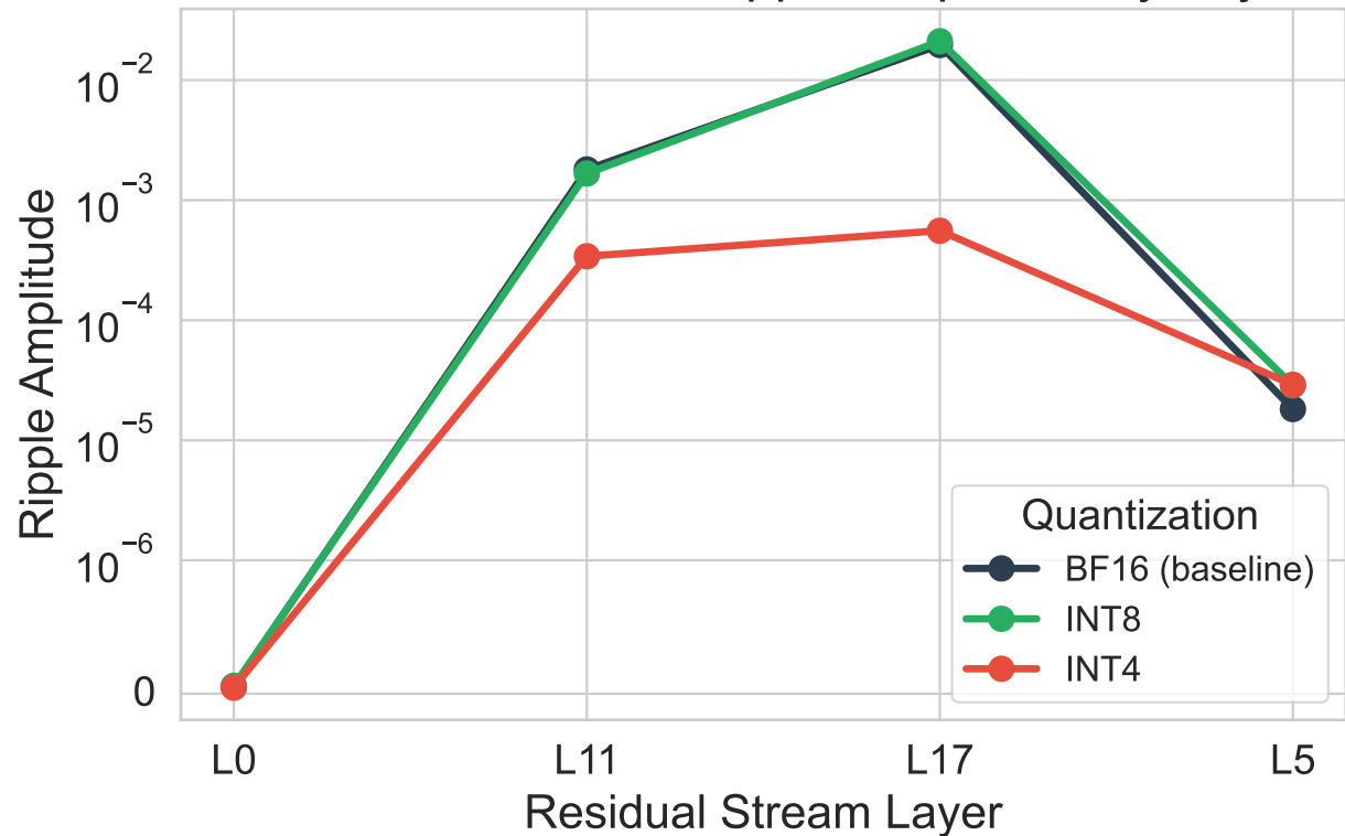
Arithmetic Manifold: Ripple Amplitude by Layer
