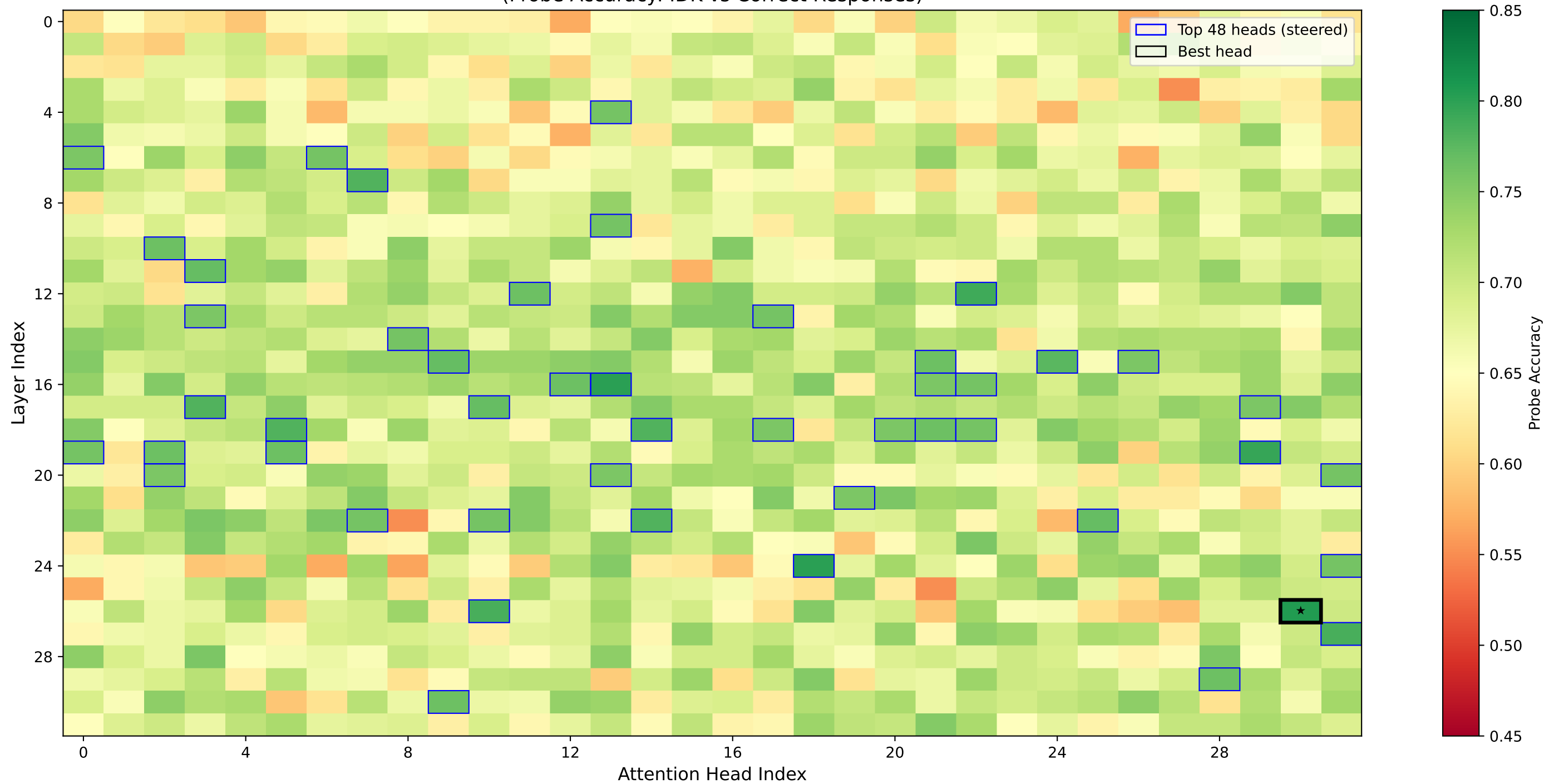
Truth-Sensitivity of Attention Heads (Probe Accuracy: IDK vs Correct Responses)
