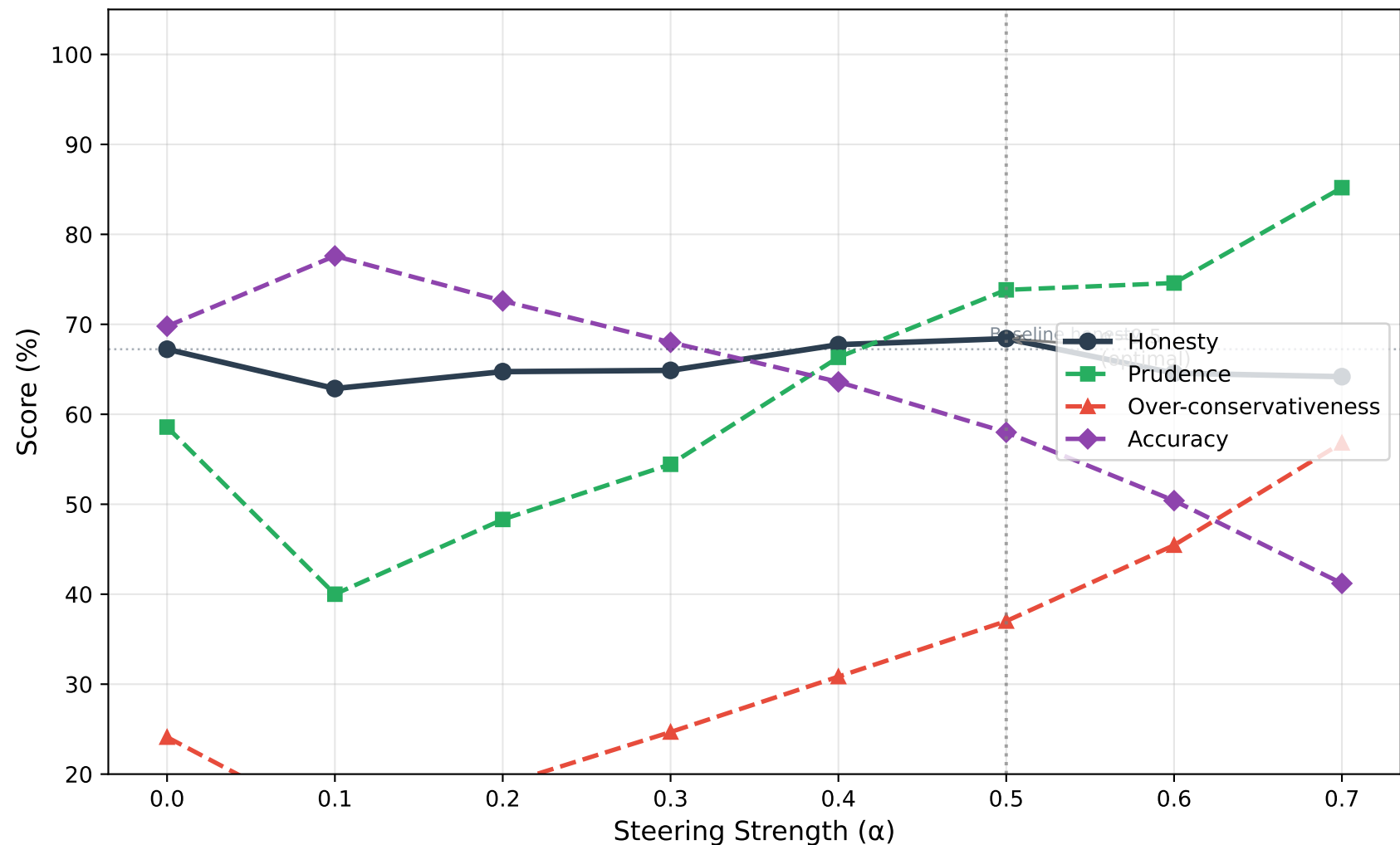
ITI Steering: Confidence-Num Model (TriviaQA, n=500)
