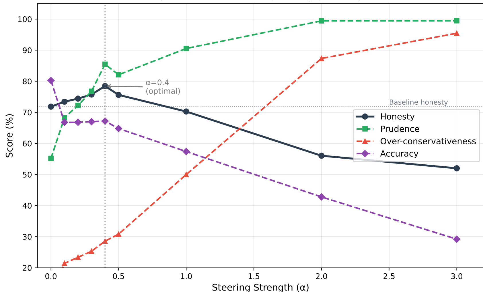
ITI Steering: Effect of Alpha on Honesty Metrics (Probe-Absolute Model, TriviaQA, n=500)
