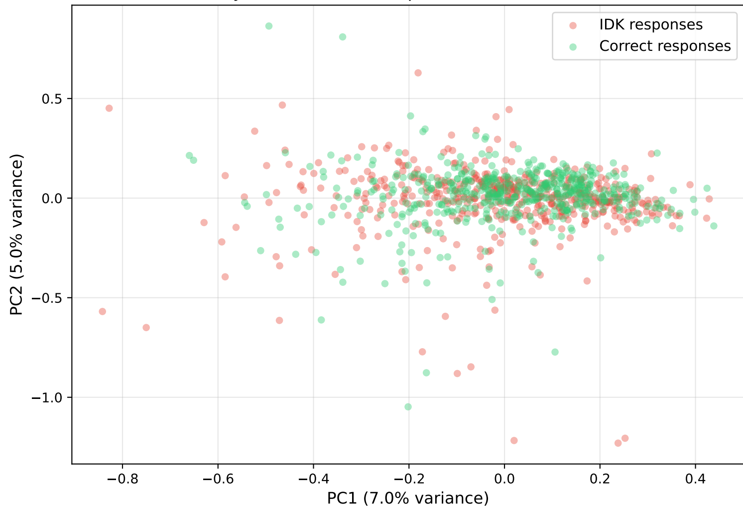
PCA of Attention Head Activations (Layer 25, Head 5 — Top Truth-Sensitive Head)
