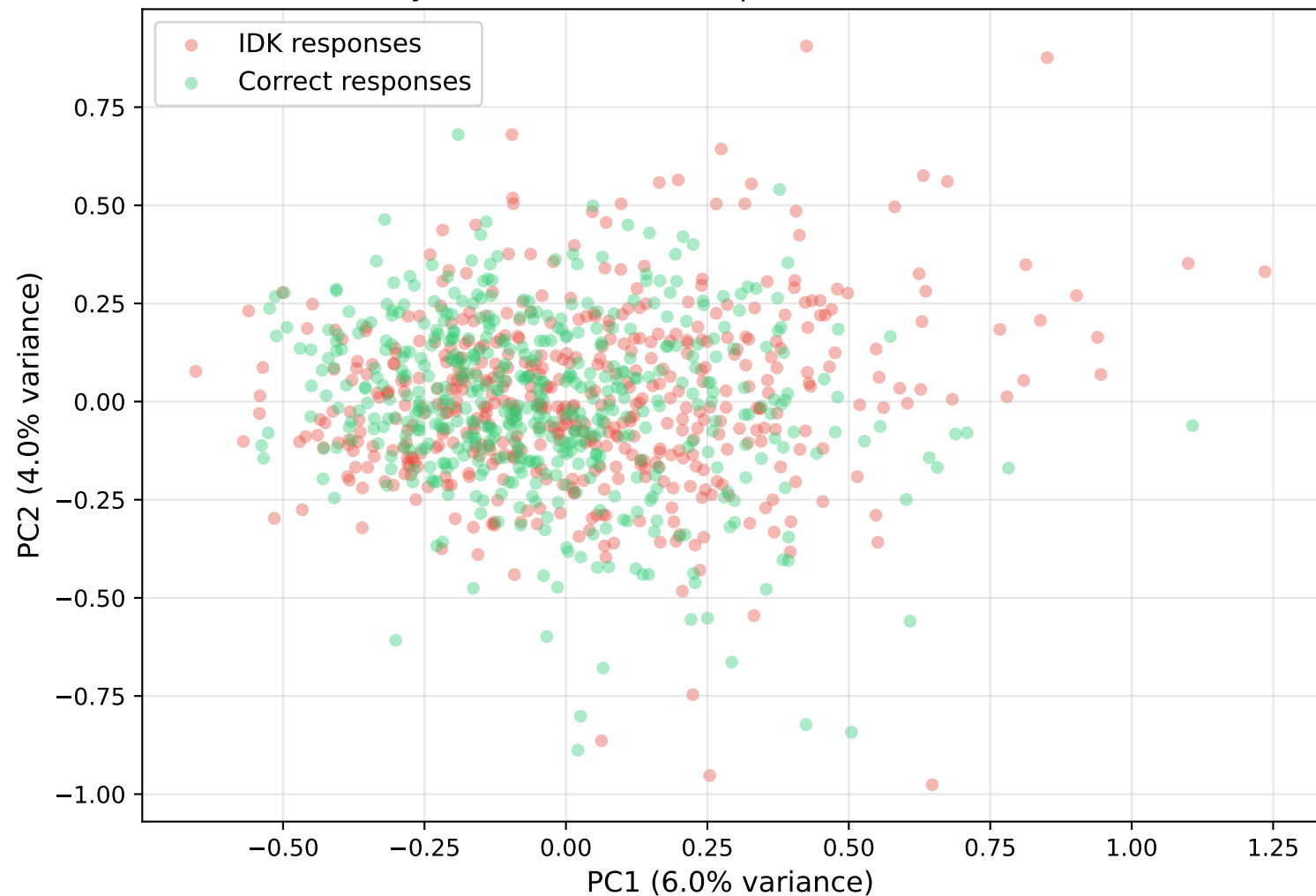
PCA of Attention Head Activations (Layer 26, Head 30 — Top Truth-Sensitive Head)
