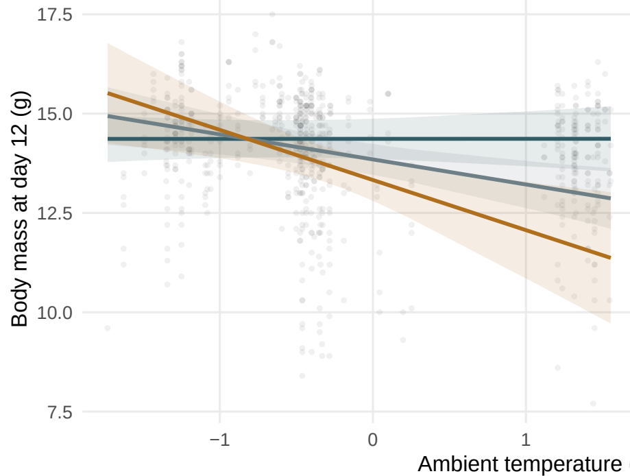
A. Incubation temperature effect at different nestling-stage temperatures
