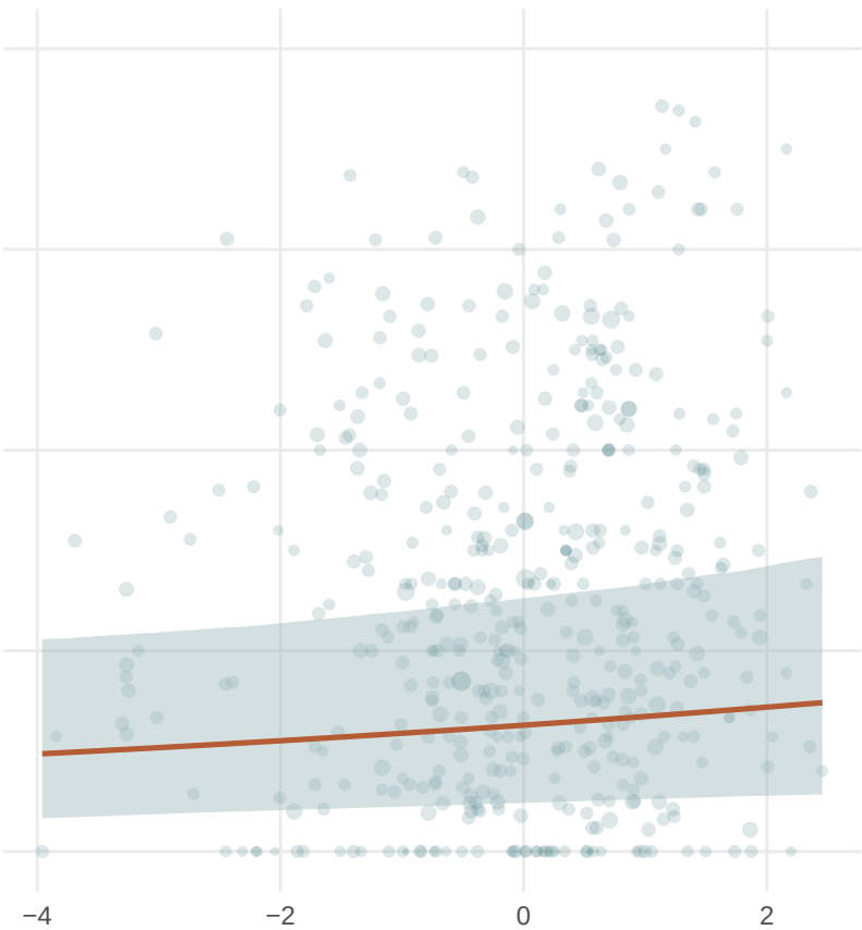
B. PC2 wet-productivity gradient
