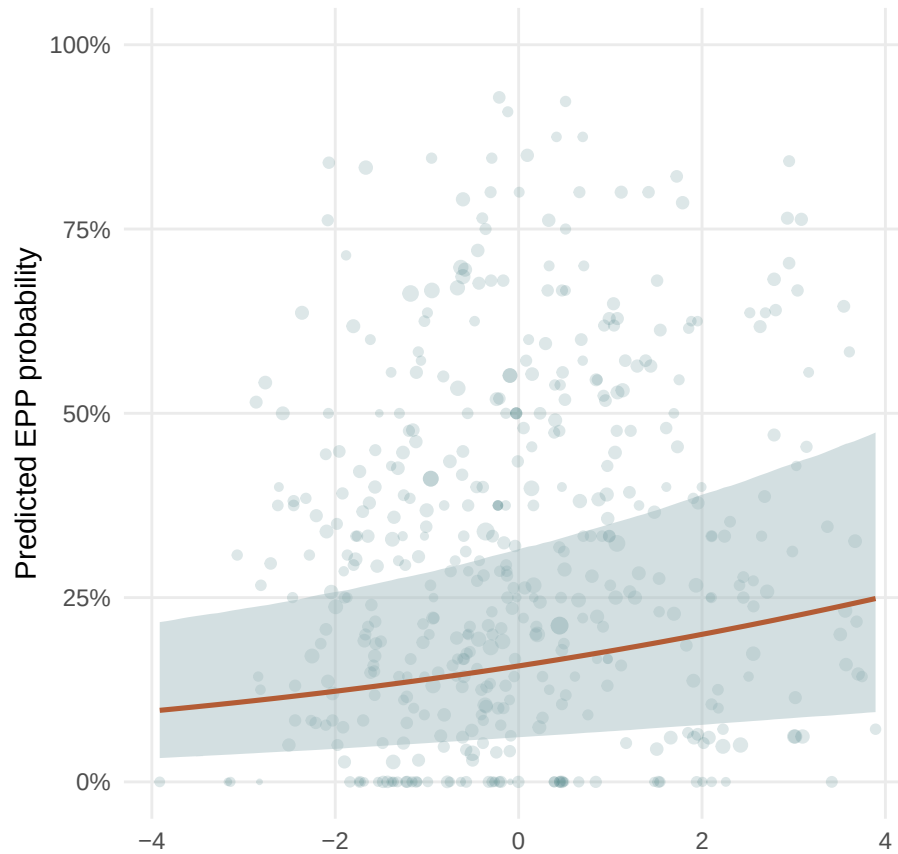
A. PC1 thermal-geographic gradient
