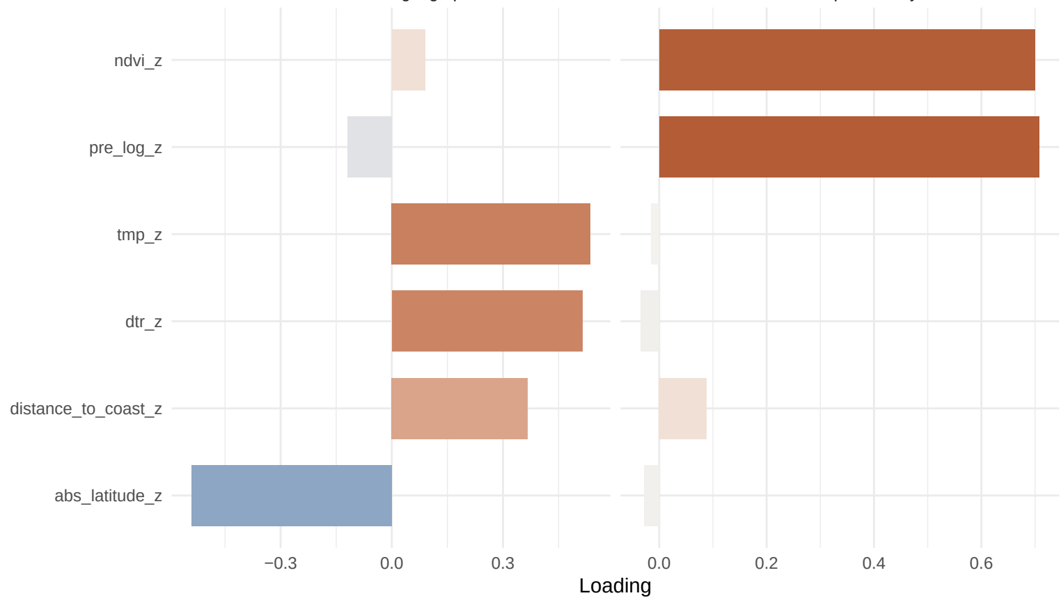
PC1 thermal-geographic
