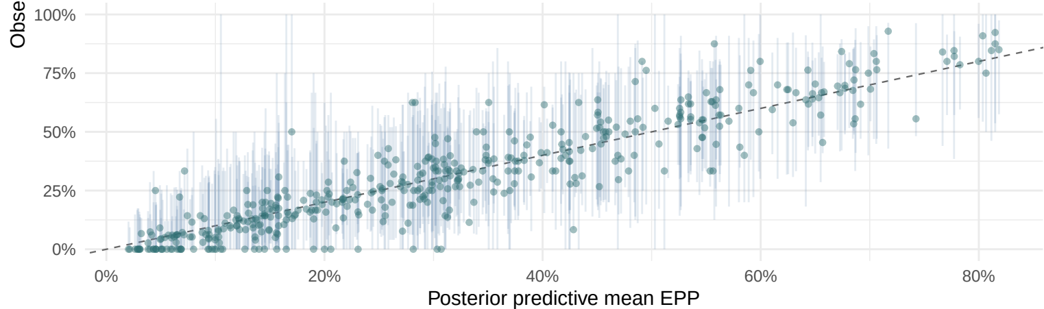
Mean-scale sensitivity
