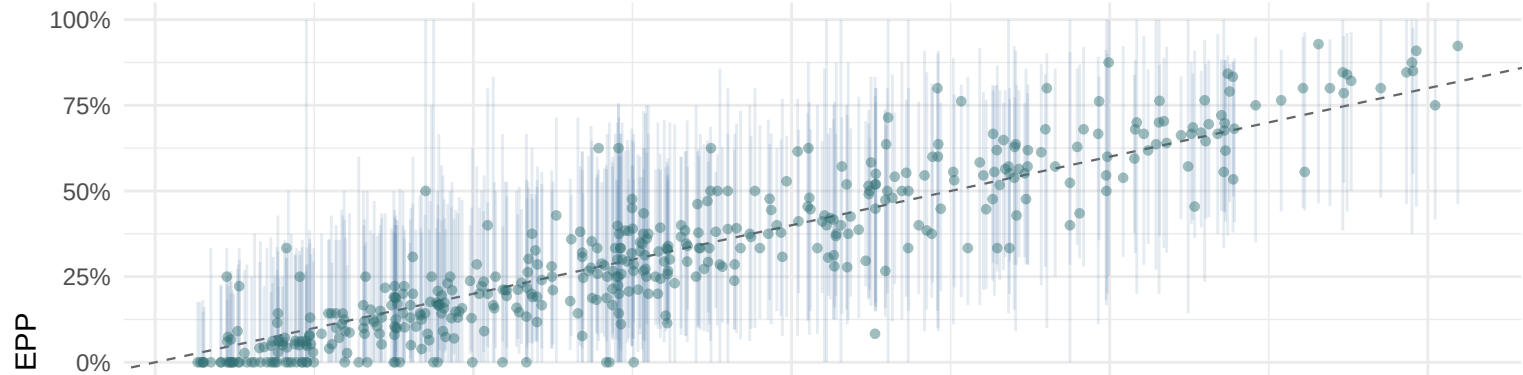
Mean-scale sensitivity
