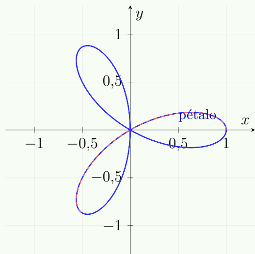
Rosa r = \cos(3\theta) , 3 pétalos
