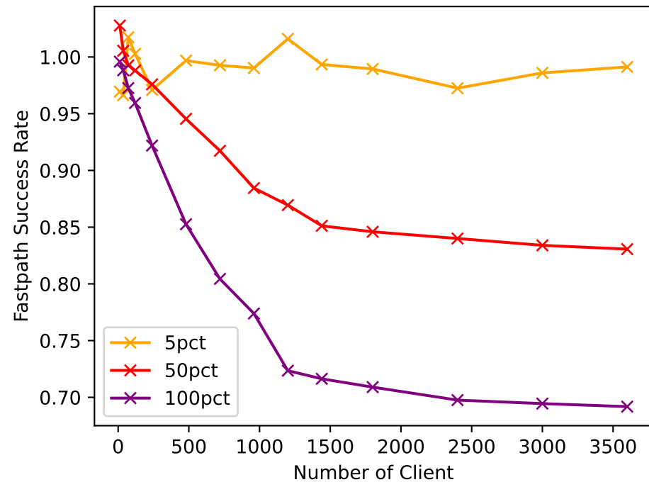
Copilot-related Fastpath Success Rate
