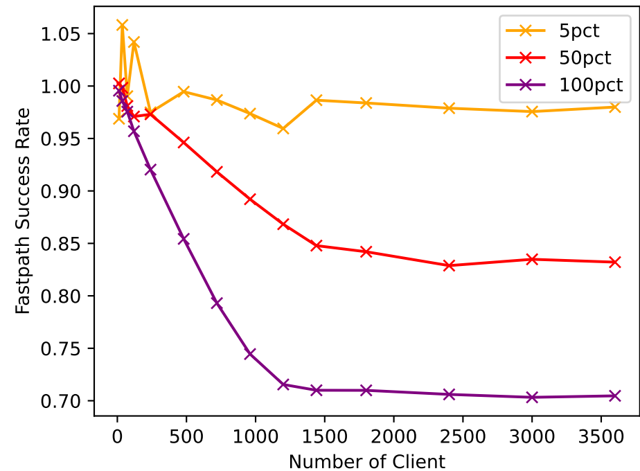
Raft-related Fastpath Success Rate
