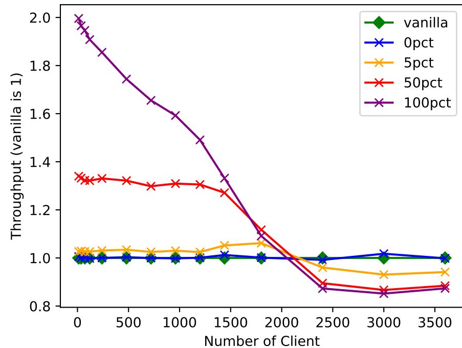
Raft-related Throughput
