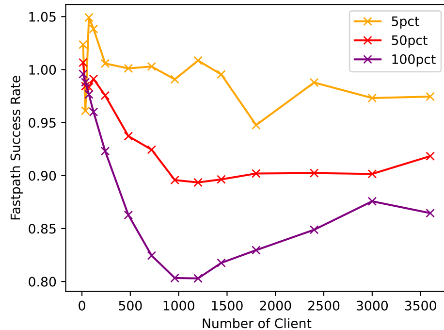
Mencius-related Fastpath Success Rate
