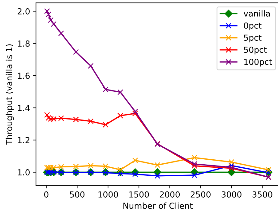
Copilot-related Throughput
