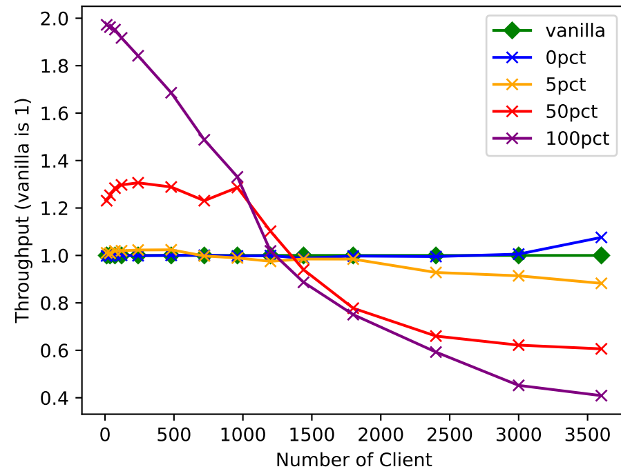
Mencius-related Throughput
