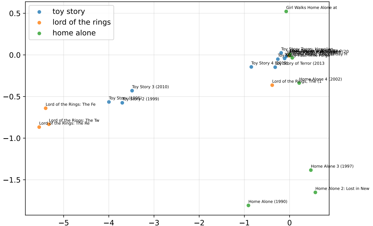
Embeddings of Selected Movies
