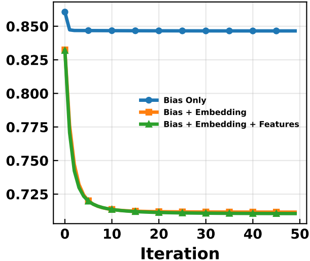
Train RMSE
