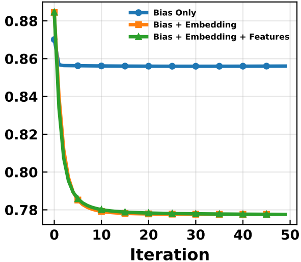
Test RMSE
