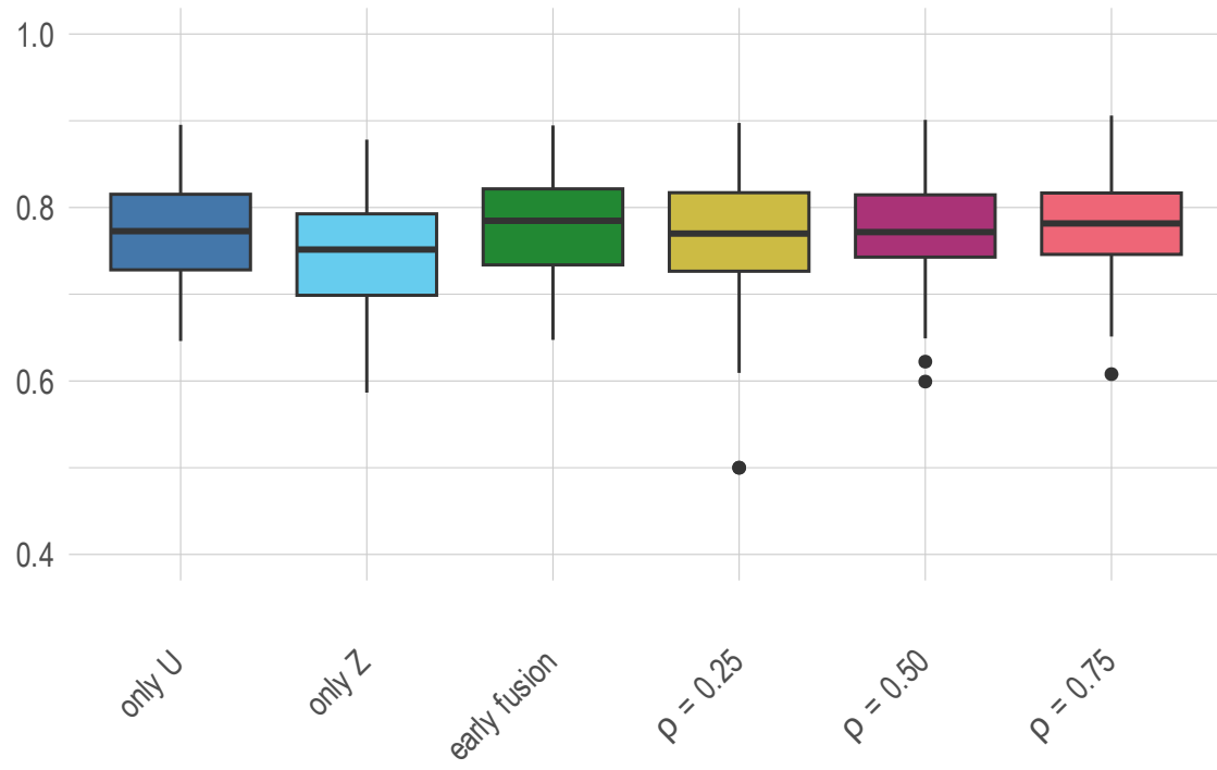
Harrell's C-index
