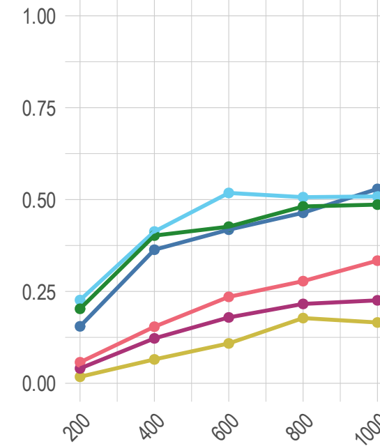
FNR
