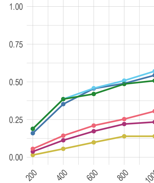
FNR
