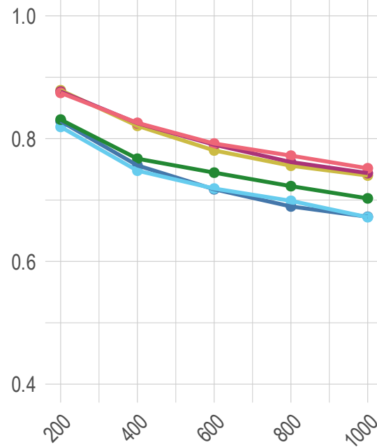
Uno's C-index
