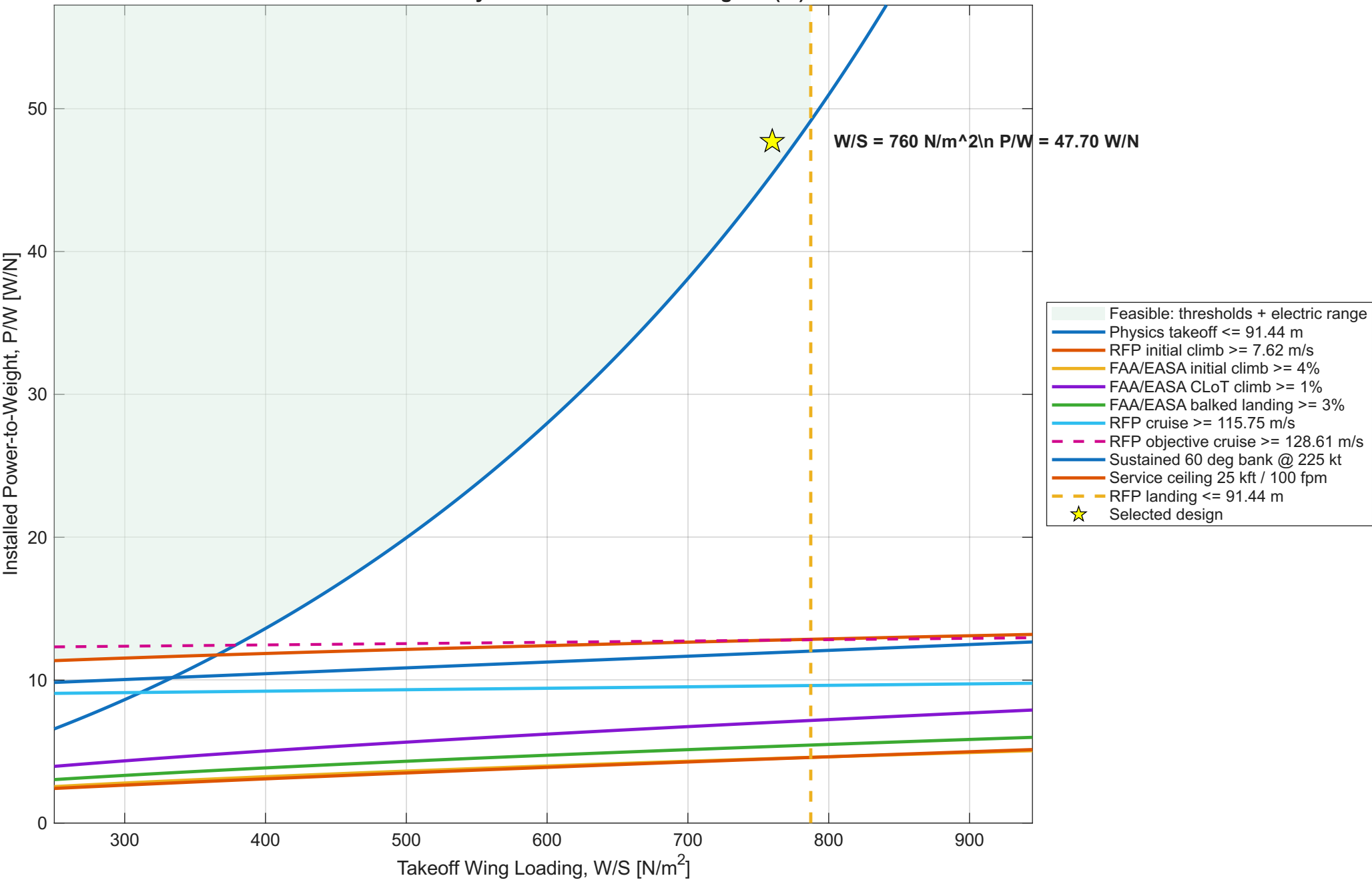
M-BRAER Preliminary P/W - W/S Constraint Diagram (SI)
