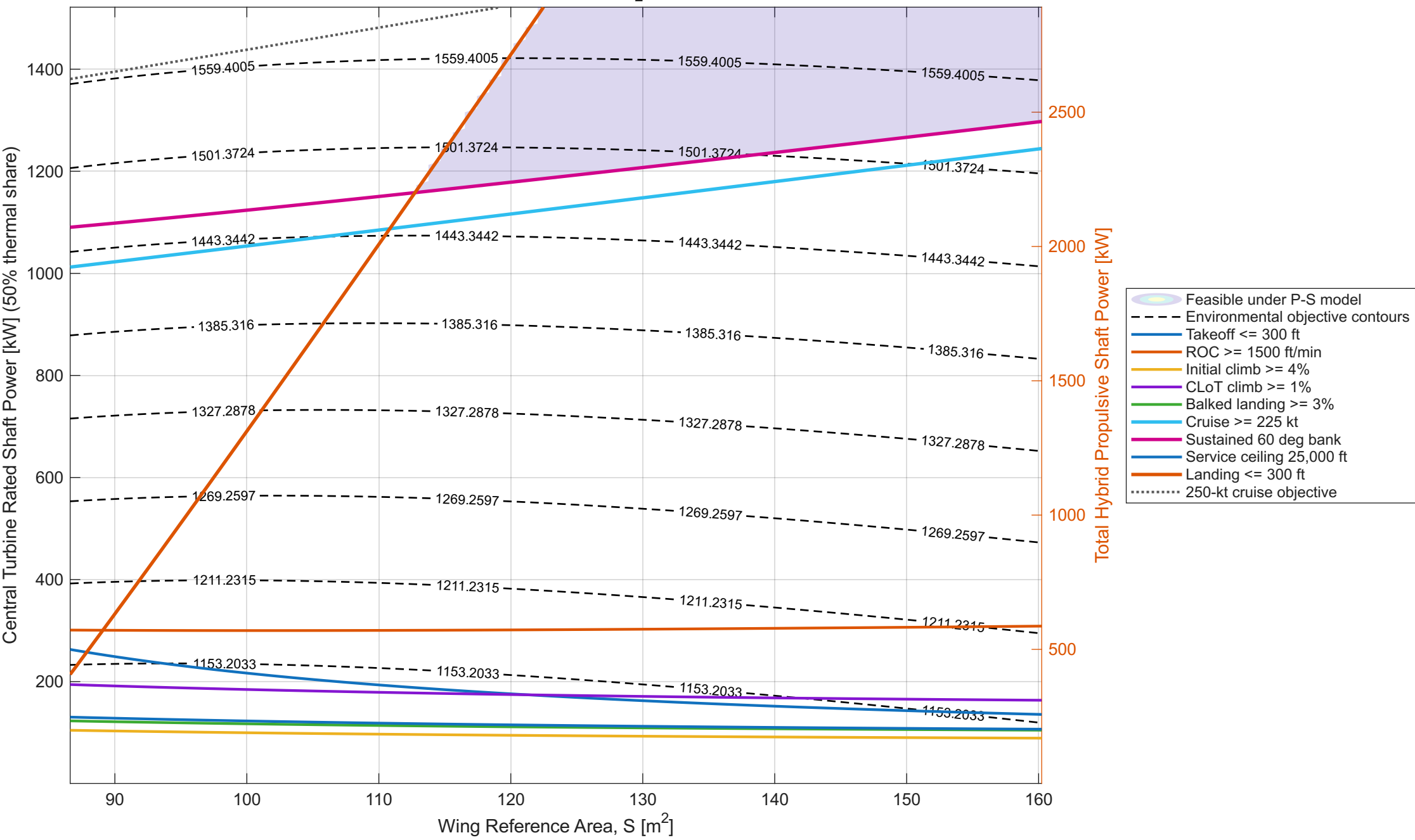
M-BRAER Parametric P-S Constraint Diagram Environmental objective contours = kg CO 2 e per mission equivalent
