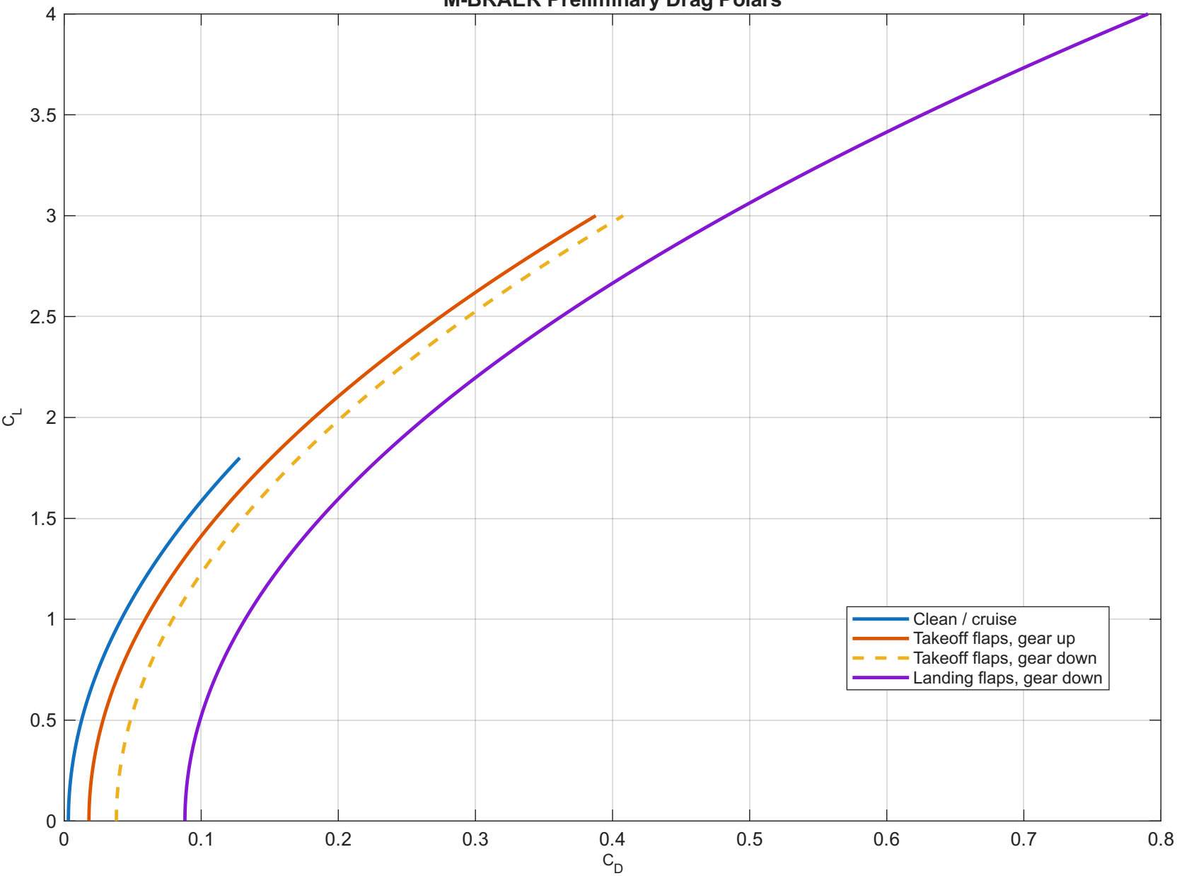
M-BRAER Preliminary Drag Polars
