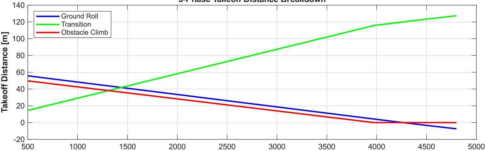
3-Phase Takeoff Distance Breakdown
