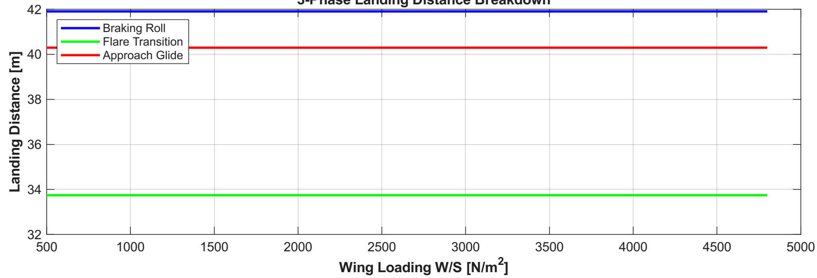
3-Phase Landing Distance Breakdown
