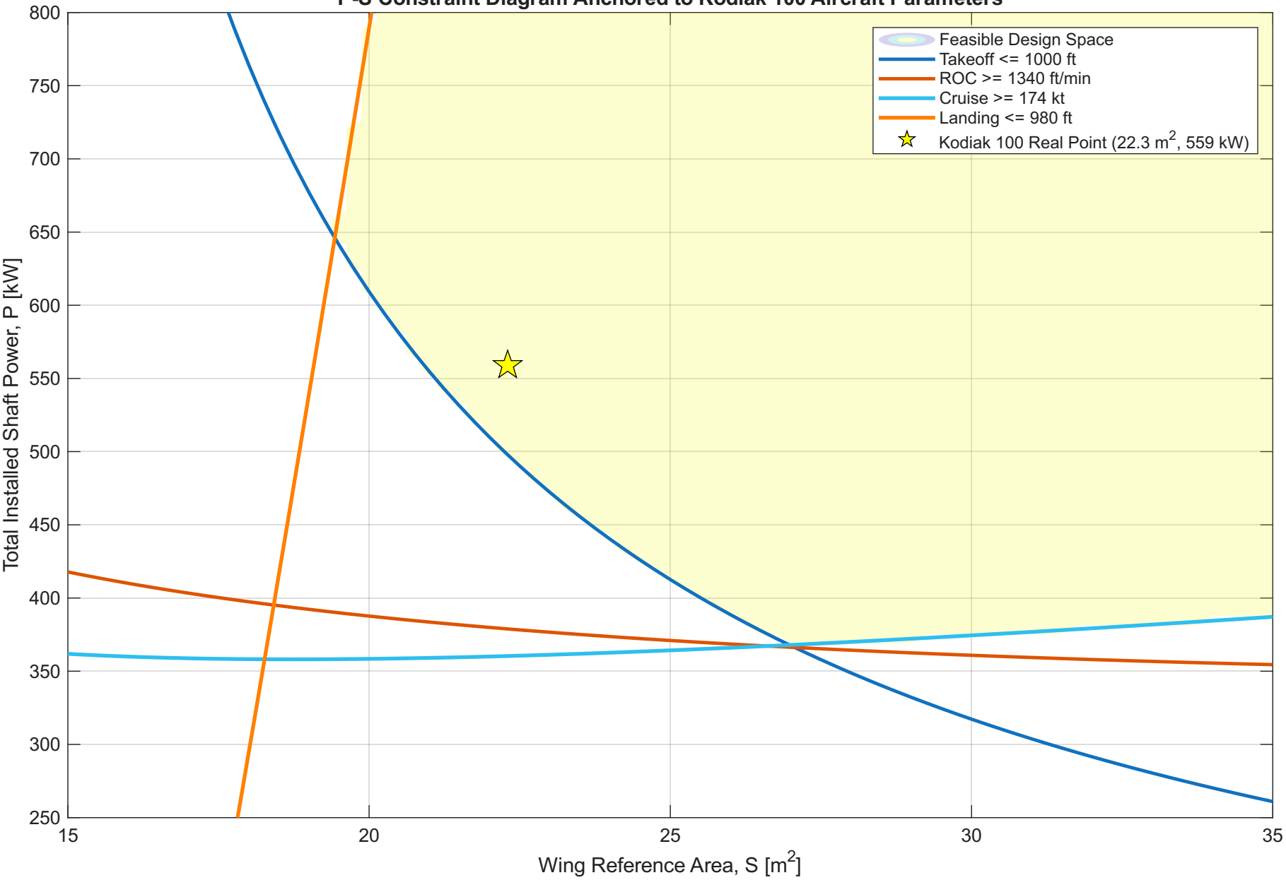
P-S Constraint Diagram Anchored to Kodiak 100 Aircraft Parameters
