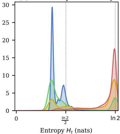
(b) AF-TKD — phases stratify
