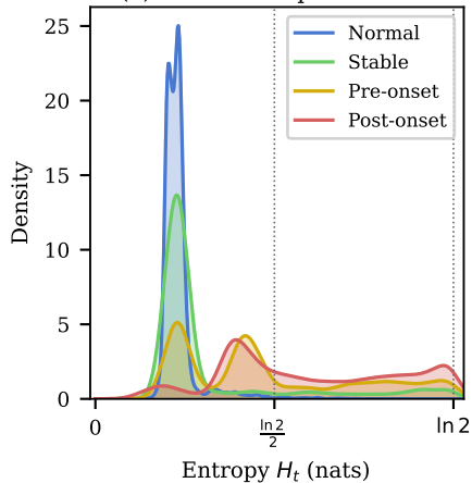
(a) Baseline — phases blur
