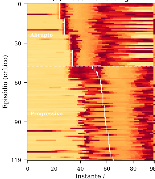
(a) Baseline+Gating
