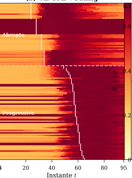
(b) AF-TKD+Gating
