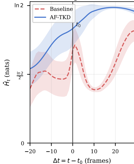
(c) \bar{H}_t \pm \frac{1}{2}\sigma around t_0
