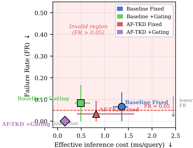
Coverage-efficiency trade-off (LSTM, 4 seeds)
