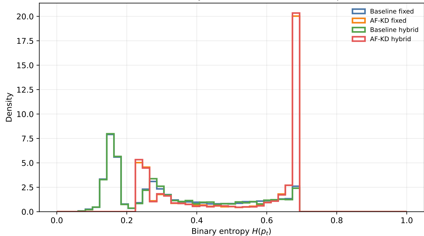
Frame-level uncertainty distribution across critical episodes
