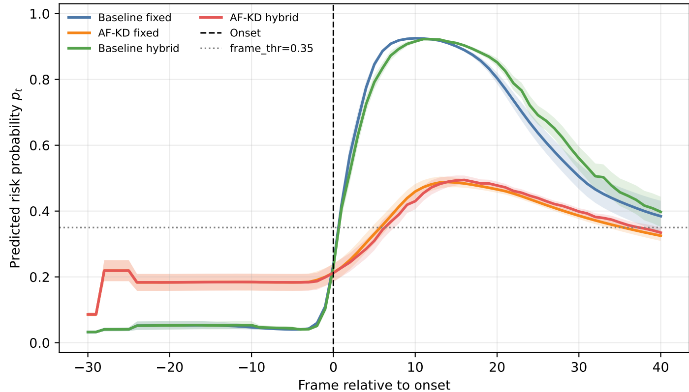
Temporal confidence trajectory around onset (abrupt)
