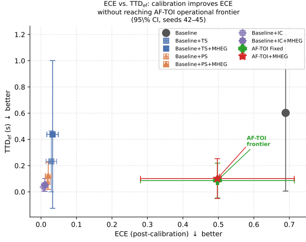
Figure 13: ECE–TTD er operational locus (CI 95%, seeds 42–45) for Baseline, post-hoc calibration variants, and AF-TOI.
