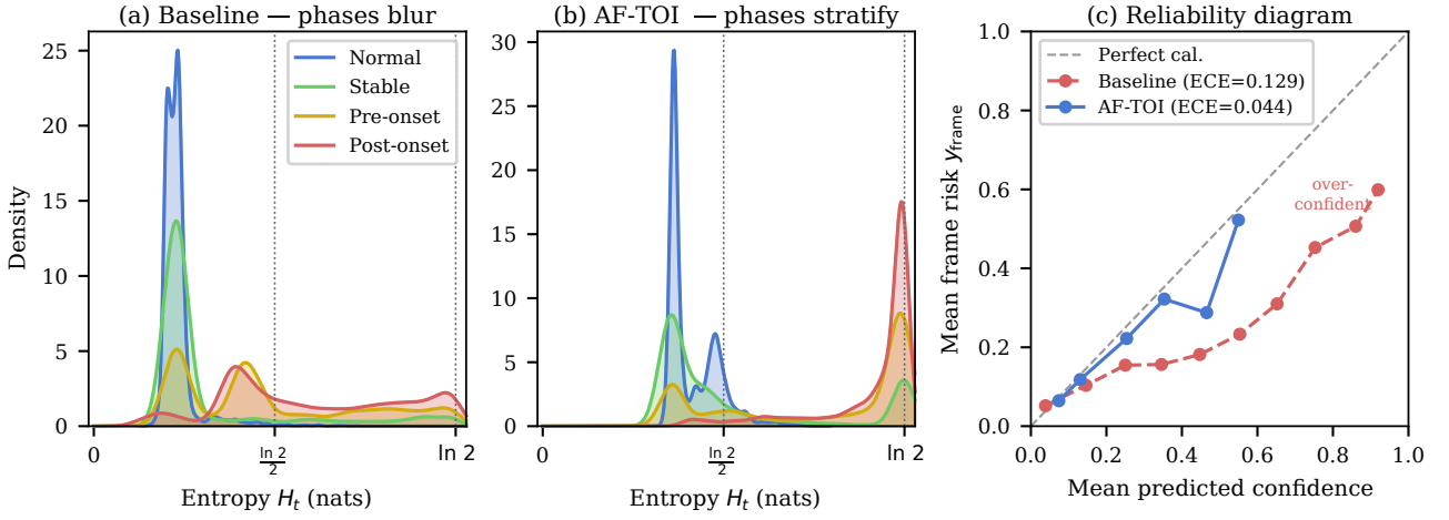
Figure 4: Trajectory organization across driving phases for seed 42. Panels compare Baseline entropy structure, AF-TOI-induced phase stratification, and frame-level calibration alignment ( ECE_{\text{frame}} = 0.044 vs. 0.129 for Baseline).
