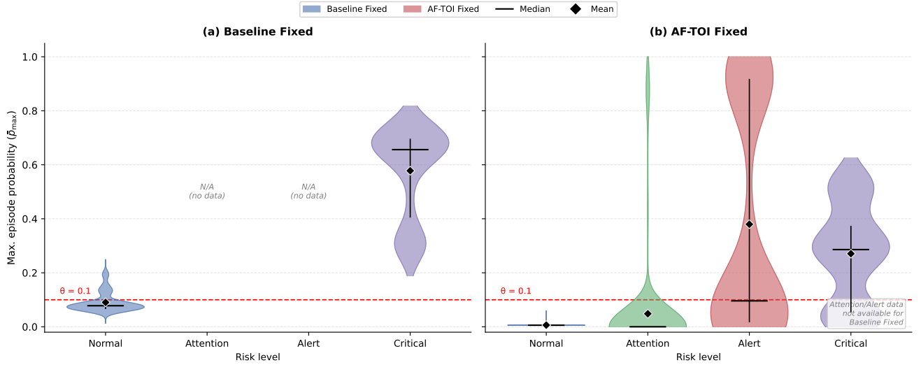
Figure 11: \bar{p}_{max} distributions by severity level in borderline episodes for seed 42. Baseline Fixed contains Normal and Critical levels; AF-TOI Fixed includes Normal, Attention, Alert, and Critical levels with activation fractions reported in the plot.
