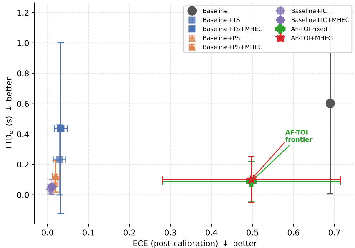
ECE vs. \text{TTD}_{\text{ef}} : calibration improves ECE without reaching AF-TOI operational frontier (95\% CI, seeds 42-45)
