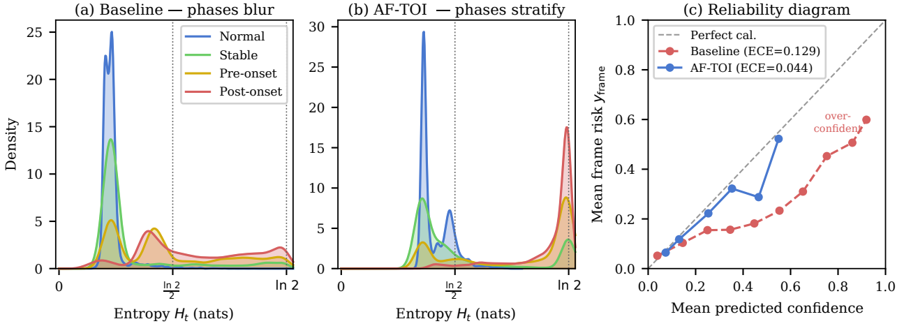
Figure 4: Trajectory organization across driving phases for seed 42. Panels compare Baseline entropy structure, AF-TOI-induced phase stratification, and frame-level calibration alignment ( \text{ECE}_{\text{frame}} = 0.044 vs. 0.129 for Baseline).
