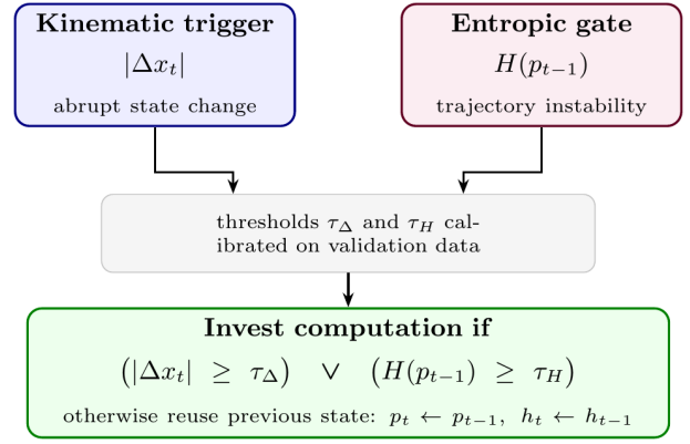
Figure 3: MHEG runtime computation scheduler structure. The kinematic component is an unconditional resource allocation trigger that forces LSTM computation whenever physical state changes abruptly, regardless of entropic state. The entropic component is the trajectory-dependent scheduling signal. When temporal organization is absent, entropy remains undifferentiated and the scheduler loses temporal discrimination power; when induced by AF-TOI, entropy stratifies near onset and the scheduler can allocate resources to emergence windows while safely suppressing redundant intervals.
