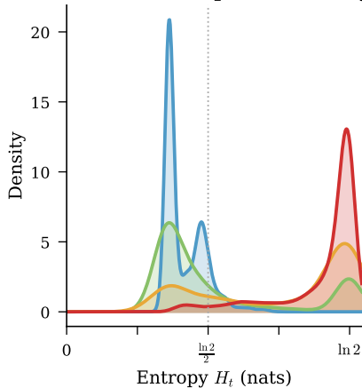
(b) AF-TKD — phases stratify
