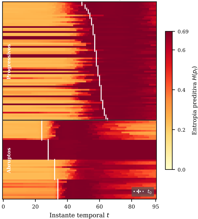
(b) LSTM-AF-TKD+Gating
