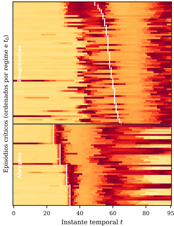
(a) LSTM-Baseline+Gating
