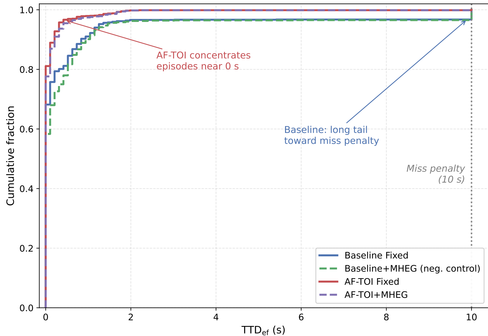
Cumulative distribution of \text{TTD}_{\text{ef}} per critical episode (seeds 42-53)
