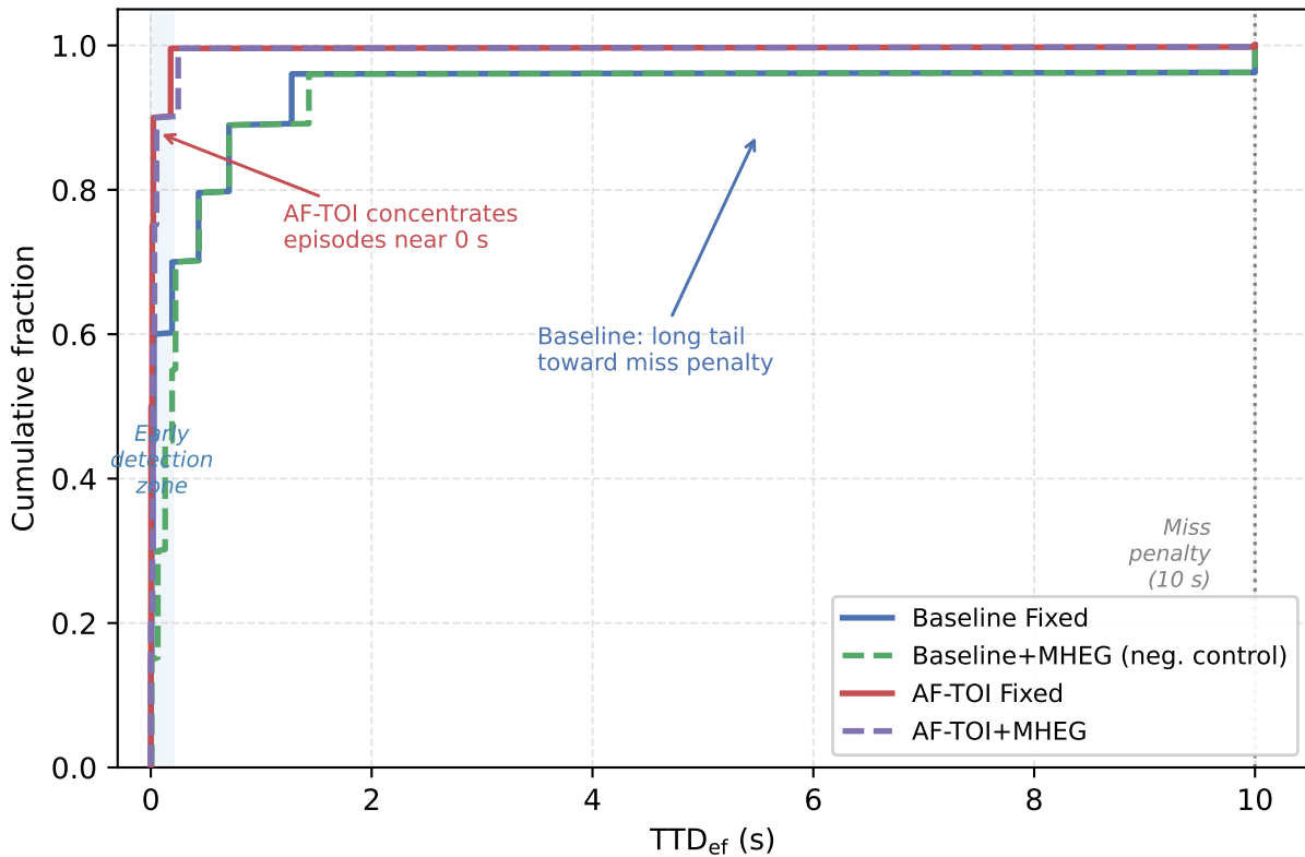
Cumulative distribution of TTD_{ef} per critical episode (seeds 42–45)
