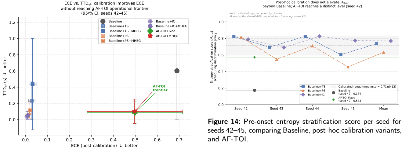
Figure 13: ECE–TTD uf operational locus (CI 95%, seeds 42–45) for Baseline, post-hoc calibration variants, and AF-TOI.
