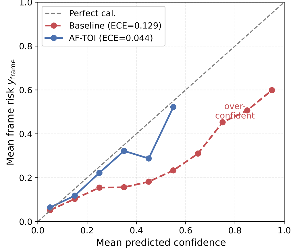
(c) Reliability diagram
