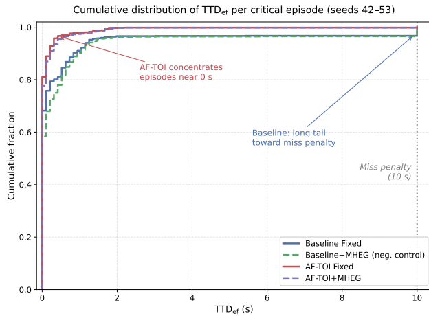
Figure 9: Cumulative distribution functions of TTD_{ef} per critical episode across seeds 42–53 ( n = 1,440 per configuration; twelve-seed campaign).
