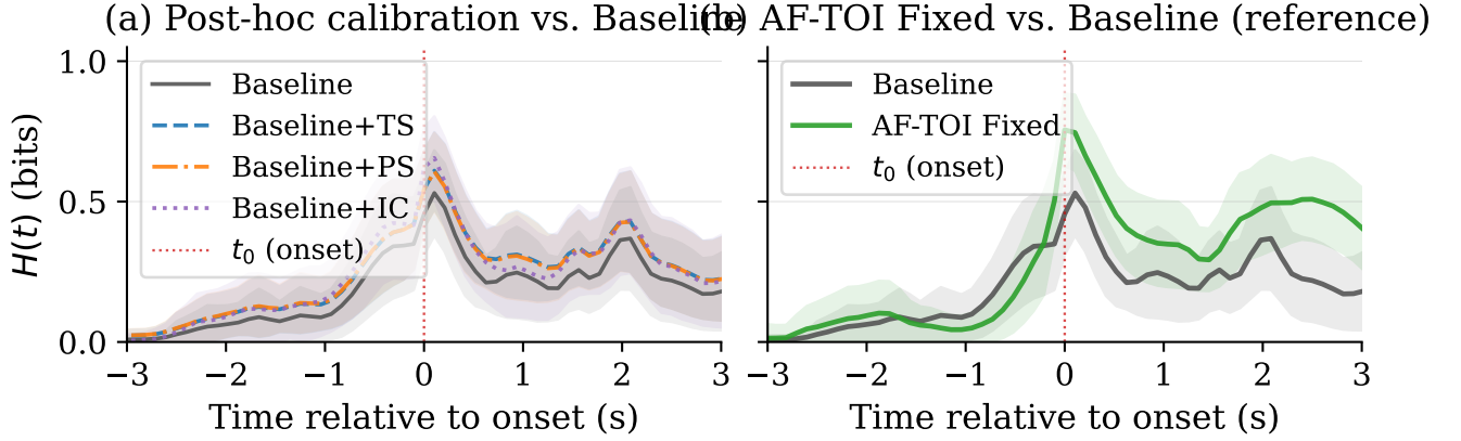
Figure 12: Mean entropy trajectory H(t) around onset for seed 42; aggregate H_{pre} metrics are consistent across seeds 42–45. Panel (a) shows post-hoc calibration variants; panel (b) shows AF-TOI.
