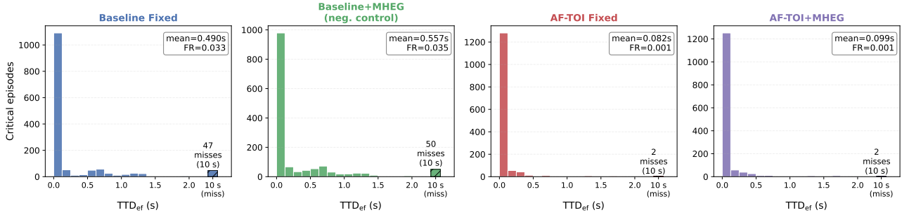
Figure 8: TTD_{ef} frequency distributions per critical episode across seeds 42–53 ( n = 1,440 per configuration). The 10 s value denotes the miss penalty used in TTD_{ef} . The in-panel mean is the per-episode average (detected delay, or 10 s when missed) and therefore differs slightly from the seed-level TTD_{ef} of Table 8, which averages the detected delay and adds FR \times T_{ep} at seed level.
