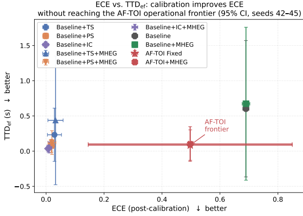
Figure 13: ECE– TTD_{ef} operational locus (CI 95%, seeds 42–45) for Baseline, post-hoc calibration variants, and AF-TOI.
