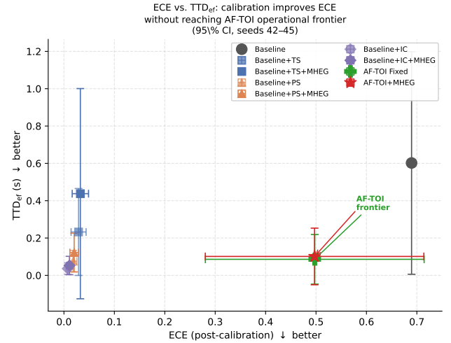
Figure 13: ECE– \text{TTD}_{\text{ef}} operational locus (CI 95%, seeds 42–45) for Baseline, post-hoc calibration variants, and AF-TOI.
