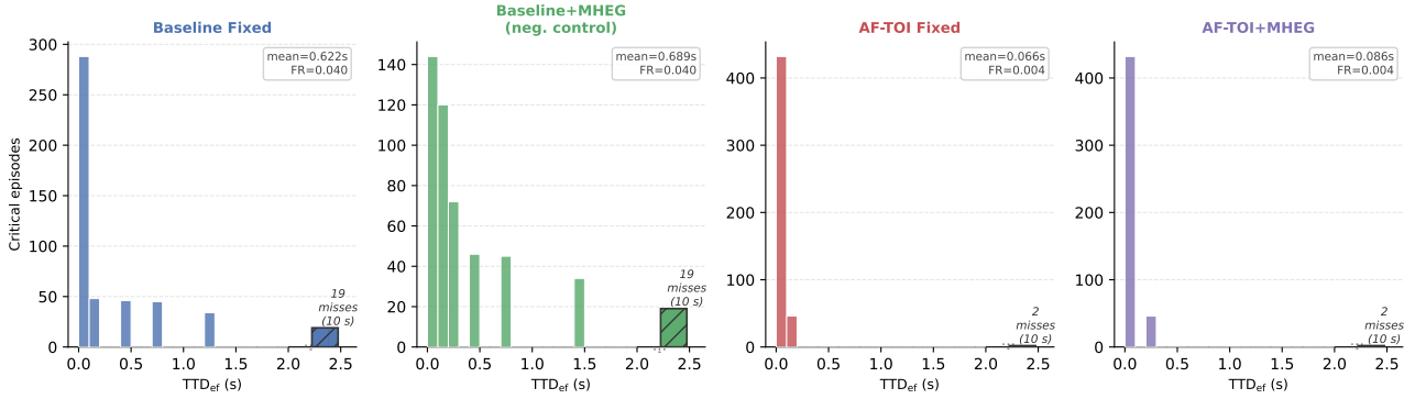
Figure 8: TTD ef frequency distributions per critical episode across seeds 42–45 ( n = 480 per configuration; original four-seed campaign, see text for the twelve-seed counts). The 10 s value denotes the miss penalty used in TTD ef .
