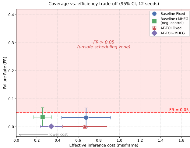
Figure 7: Global miss rate versus effective inference cost per frame (CI 95%, seeds 42–53). The dashed line marks the FR = 0.05 safety boundary; the shaded area denotes the unsafe scheduling region.
