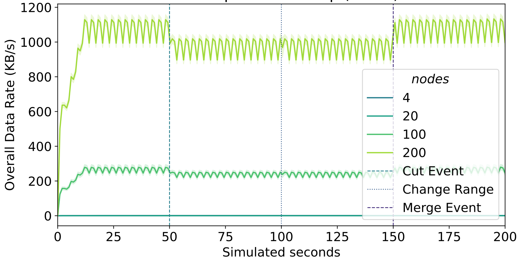
Time Replicated Gossip (MinOf)
