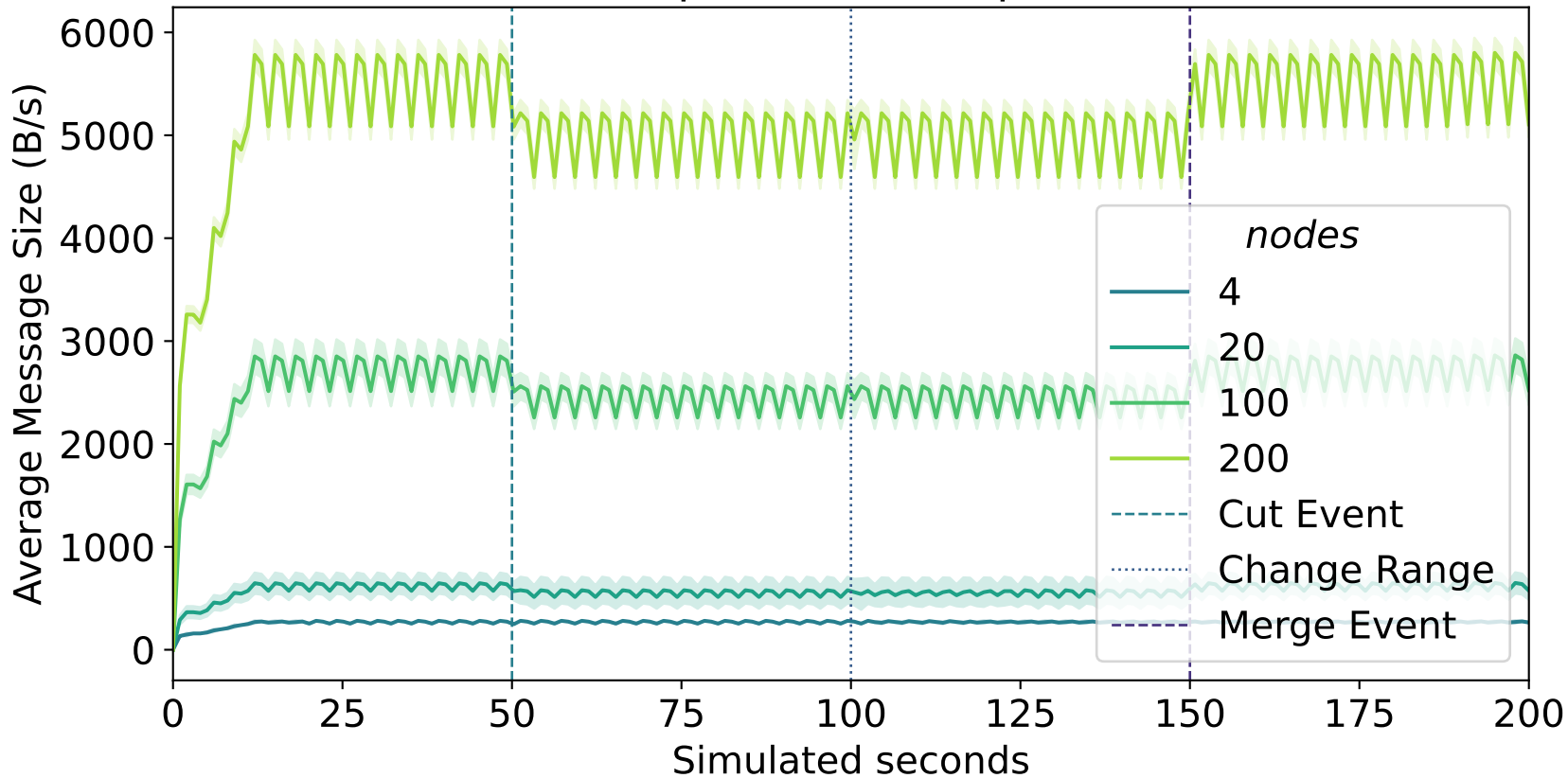
Time Replicated Gossip (MinOf)
