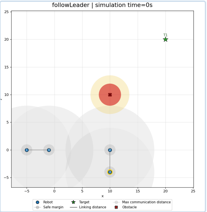
Safety CBF/CLF filter on transients
