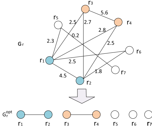
Fig. 3. An example illustrates our graph-based problem formulation: the objective is to reduce the record graph G_r to the ground-truth graph G_r^{opt} .
