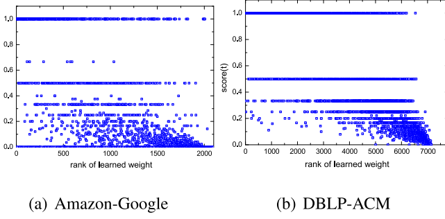
Fig. 5. Visualization of the effectiveness of the learned term weights.
