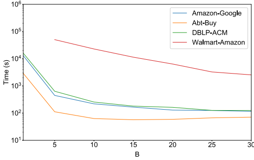
Fig. 7. Total running time with different number of blocks.
