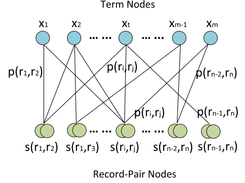
Fig. 2. An example of bipartite graph for terms and record-pairs.
