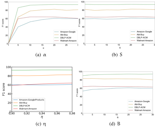
Fig. 4. Parameter sensitivity analysis for the algorithm of ITER +CliqueRank.
