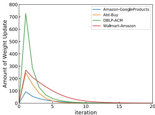
Fig. 6. Convergence of ITER algorithm.
