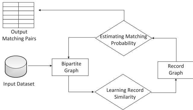
Fig. 1. An overview of our framework for unsupervised entity resolution. We will propose ITER to learn record similarity and CliqueRank to estimate matching probability.
