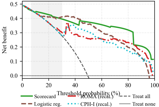
Fig. 2. Decision curve analysis on West China ( N = 380 ): net benefit against the decision threshold, with treat-all (dashed) and treat-none (horizontal axis) references; the shaded band marks the range of published cutpoints (7–30%). Scorecard and formulas are shown after within-cohort recalibration (logistic regression as fitted); XGBoost omitted.
