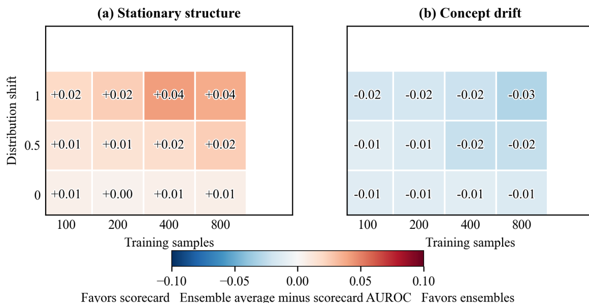
Fig. 3. Regime map from the simulation: mean over 20 replicates of the tree-ensemble-average minus scorecard test AUROC at 50% noise (red favors the ensembles, blue the scorecard); axes: training samples (100–800), distribution shift (0–1).
