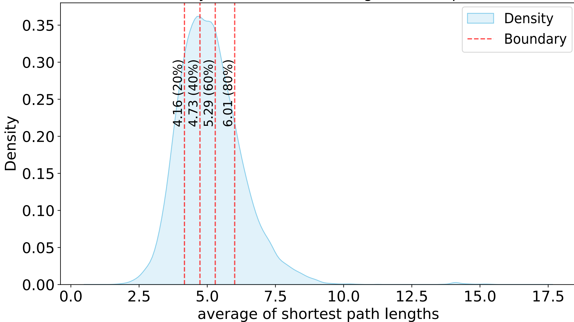
Density Distribution of average shortest path
