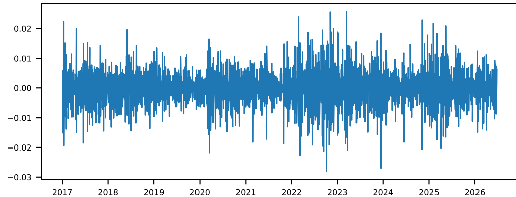
VIXCLS (1st difference) - ADF p=0.0000 [stationary]
