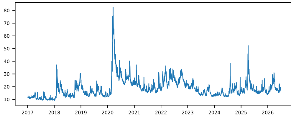
VIXCLS (level) - ADF p=0.0000 [stationary]
