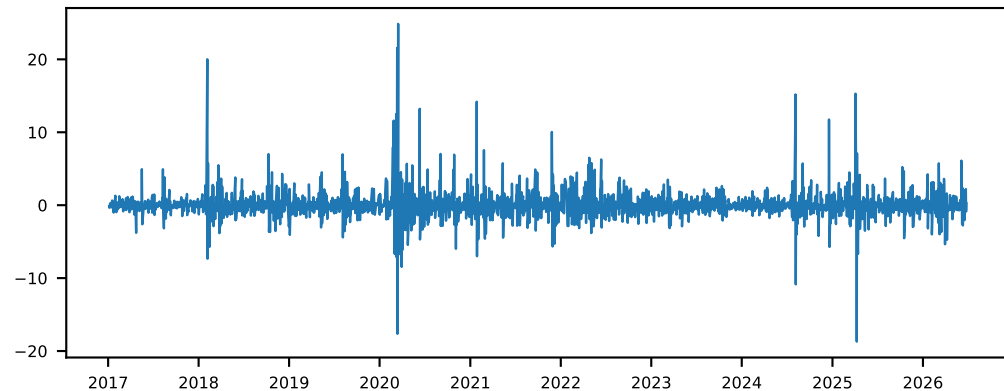
VIXCLS (1st difference) - ADF p=0.0000 [stationary]
