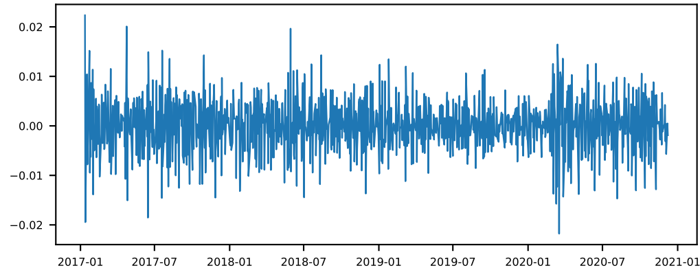
USEPUINDXD_diff (1st difference) - ADF p=0.0000 [stationary]
