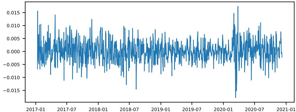
USEPUINDXD_diff (level) - ADF p=0.0000 [stationary]
