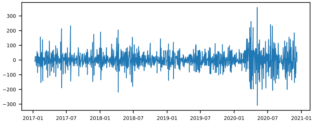
USEPUINDXD_diff (level) - ADF p=0.0000 [stationary]
