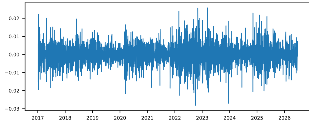
VIXCLS (1st difference) - ADF p=0.0000 [stationary]
