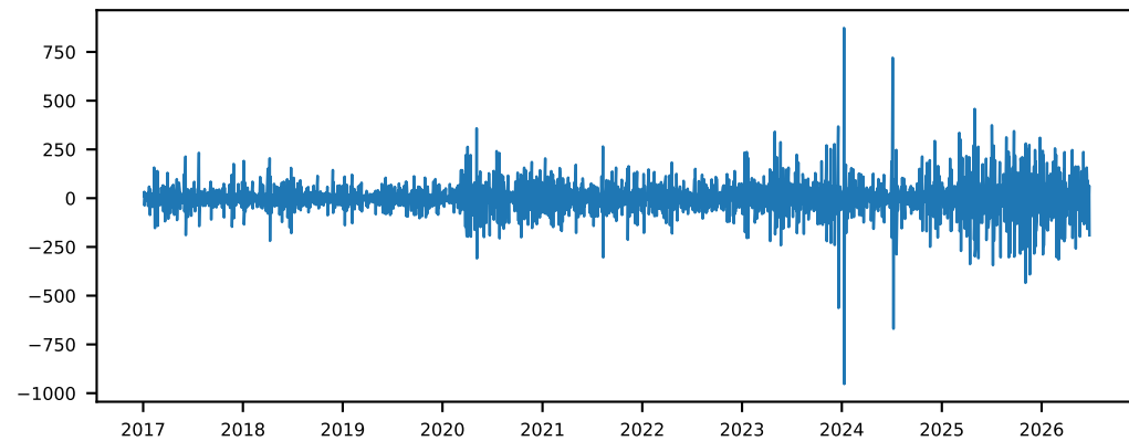
USEPUINDXD_diff (level) - ADF p=0.0000 [stationary]
