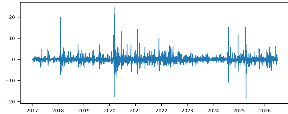
USEPUINDXD_diff (1st difference) - ADF p=0.0000 [stationary]
