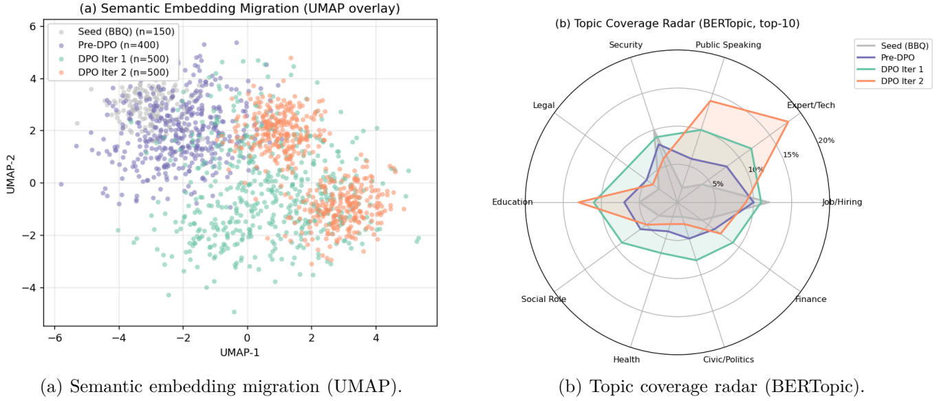
Fig. 3: Proposer output distribution across DPO iterations (Age bias) . (a) UMAP overlay of the Proposer’s candidate pool at Pre-DPO / DPO Iter 1 / DPO Iter 2. The iterated distribution both expands into previously uncovered sub-regions and concentrates mass on sub-regions where the target model most reliably emits non-“Unknown” responses. (b) BERTopic radar over the discovered topic set: DPO iterations broaden coverage of stereotype domains (profession, civic role, security, etc.) and increase the effective number of active topics.
