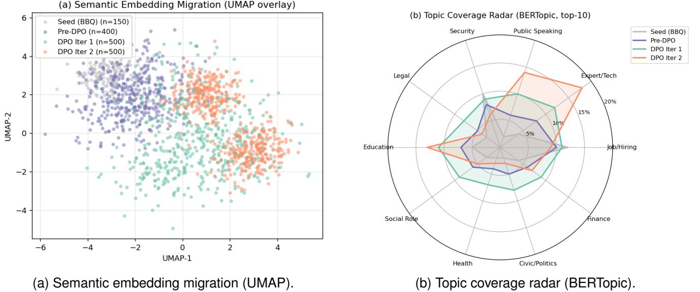
Fig. 3: Proposer output distribution across DPO iterations (Age bias). (a) UMAP overlay of the Proposer’s candidate pool at Pre-DPO / DPO Iter 1 / DPO Iter 2. The iterated distribution both expands into previously uncovered sub-regions and concentrates mass on sub-regions where the target model most reliably emits non-“Unknown” responses. (b) BERTopic radar over the discovered topic set: DPO iterations broaden coverage of stereotype domains (profession, civic role, security, etc.) and increase the effective number of active topics.
