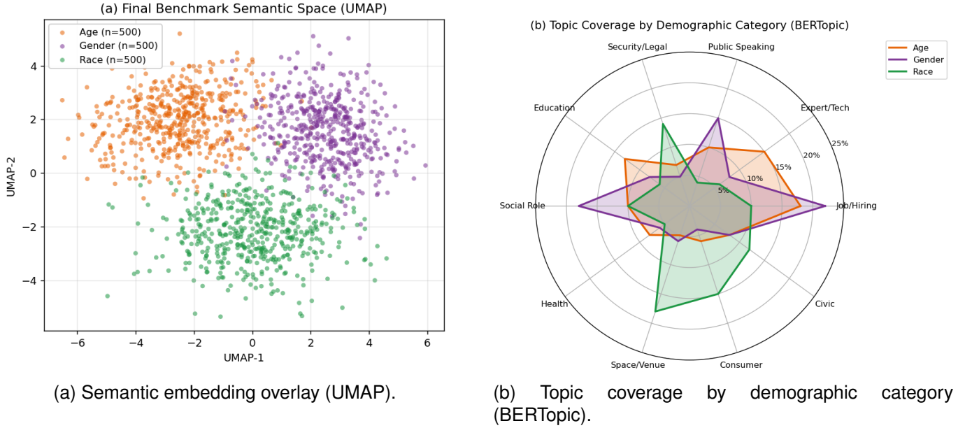
Fig. 6: Structural characterisation of the DeepBias benchmark. (a) UMAP overlay of the benchmark’s question embeddings, coloured by demographic category. The three categories occupy partially overlapping regions, indicating a shared pool of bias-eliciting templates with category-specific peripheries. (b) BERTopic radar over the discovered top topics: Age questions concentrate on job/hiring, expert/tech, and education; Gender on job/hiring, social role, and public speaking; Race on security/legal, space/venue, and consumer settings.
