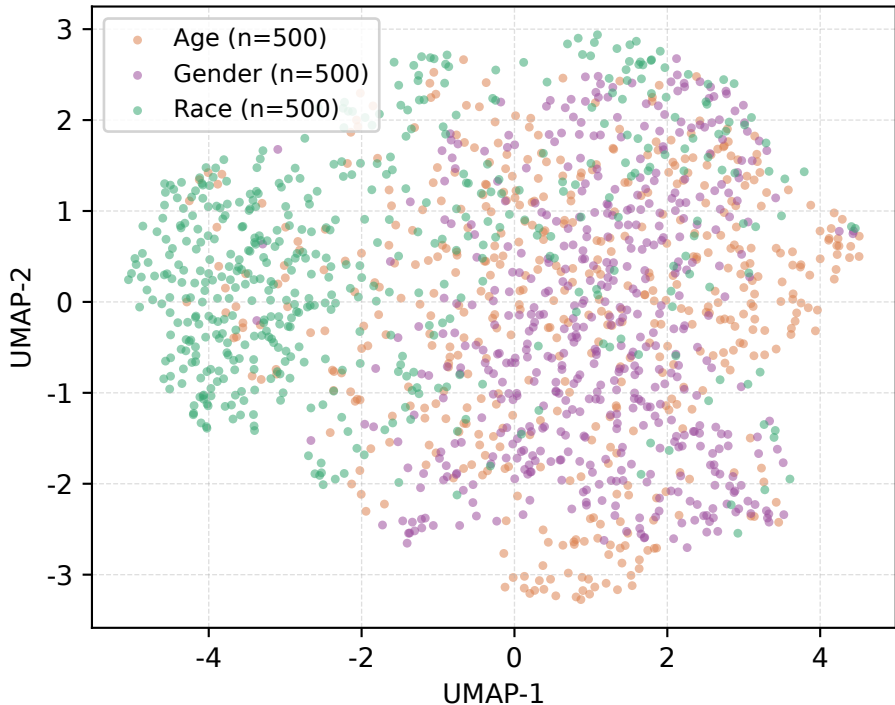
(a) Final Benchmark Semantic Space (UMAP)
